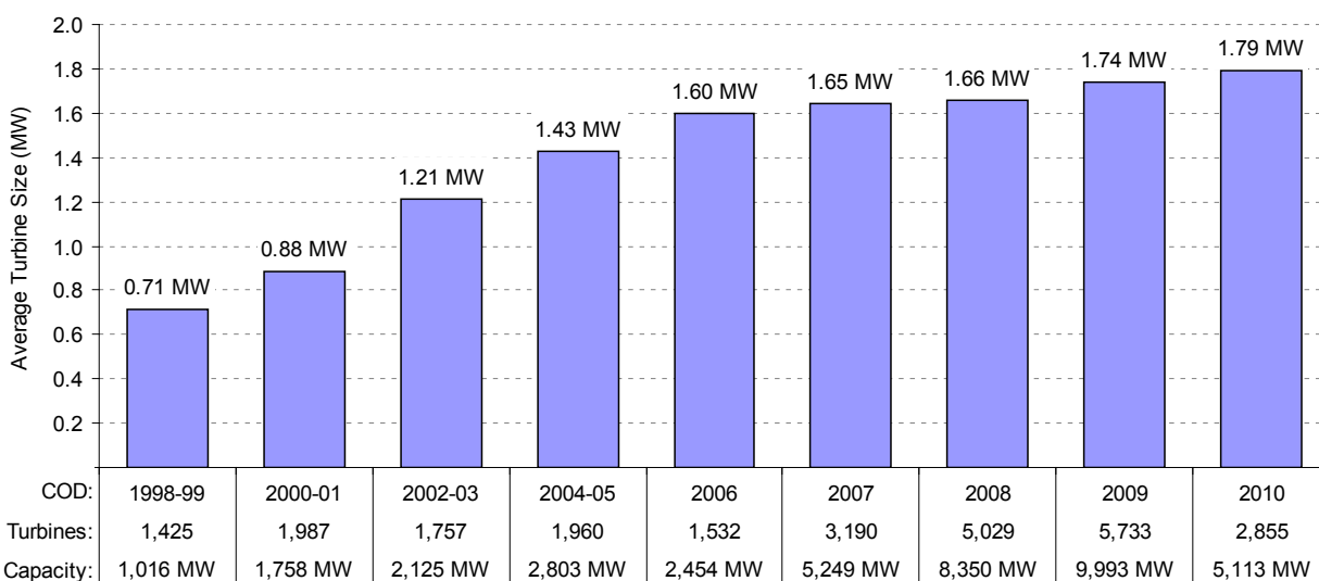
Figure 16. Average Turbine Nameplate Capacity Installed During Period
