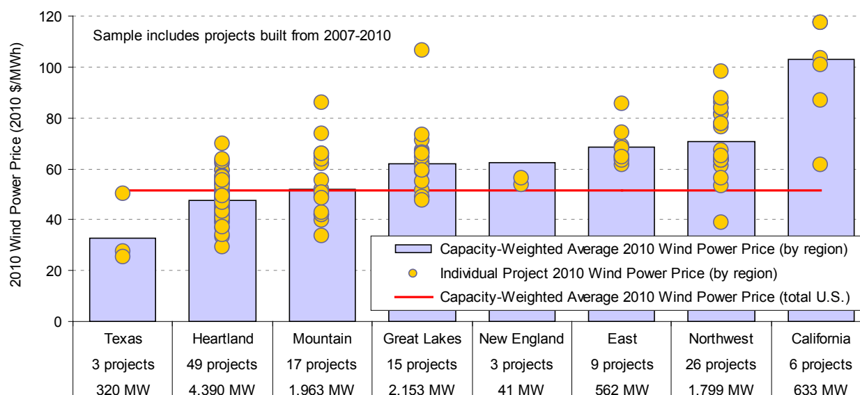
Figure 22. 2010 Wind Power Prices by Region: 2007-2010 Projects Only
