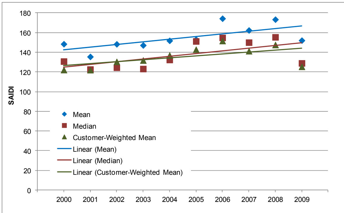
Figure 14. SAIDI without Major Events – Reported Reliability Data from Same Utilities for Every Year – N=67
