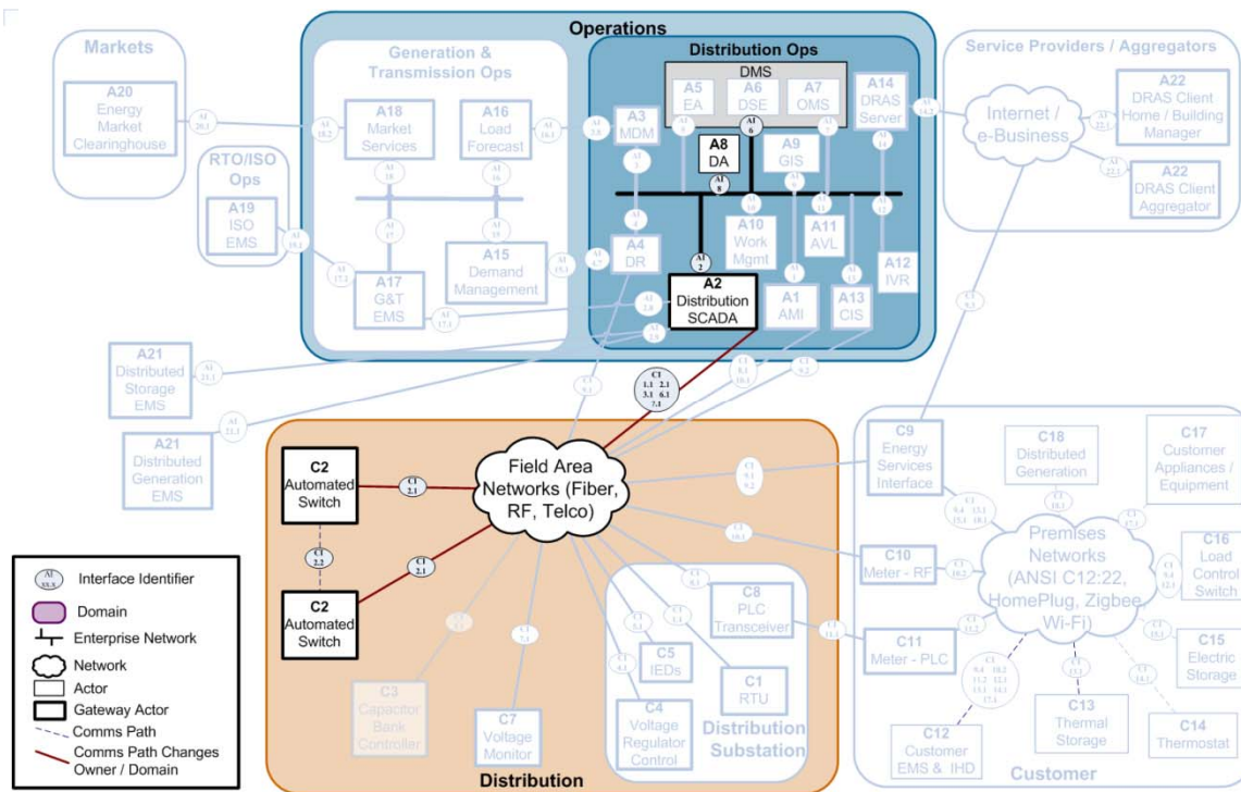
Figure 7. Smart Grid Demonstration Grant Activity Type—Smart Feeder Switching Components and Interfaces.
