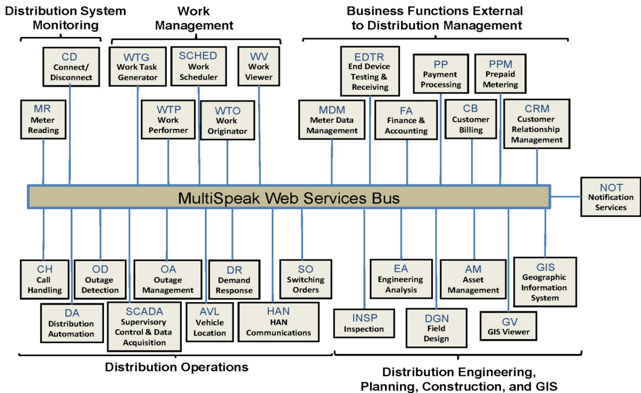
Figure 8. MultiSpeak® as an Enterprise Service Bus.
