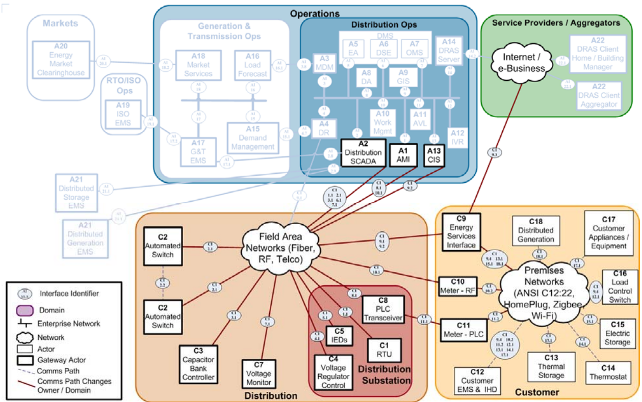
Figure 4 provides an overview of the domains, physical component (device) actors, and component interfaces that comprise our smart grid demonstration activity types. Application actors were defined in the previous section and only those to which a direct physical component interface exists are illustrated. Note that component vendors offer varying levels of integration,
