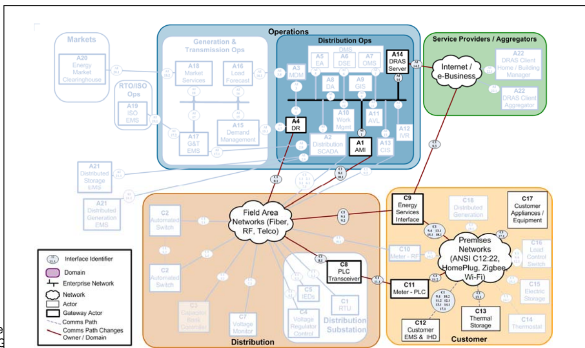
Figure 14. Interactive Thermal Storage Architecture Diagram.
