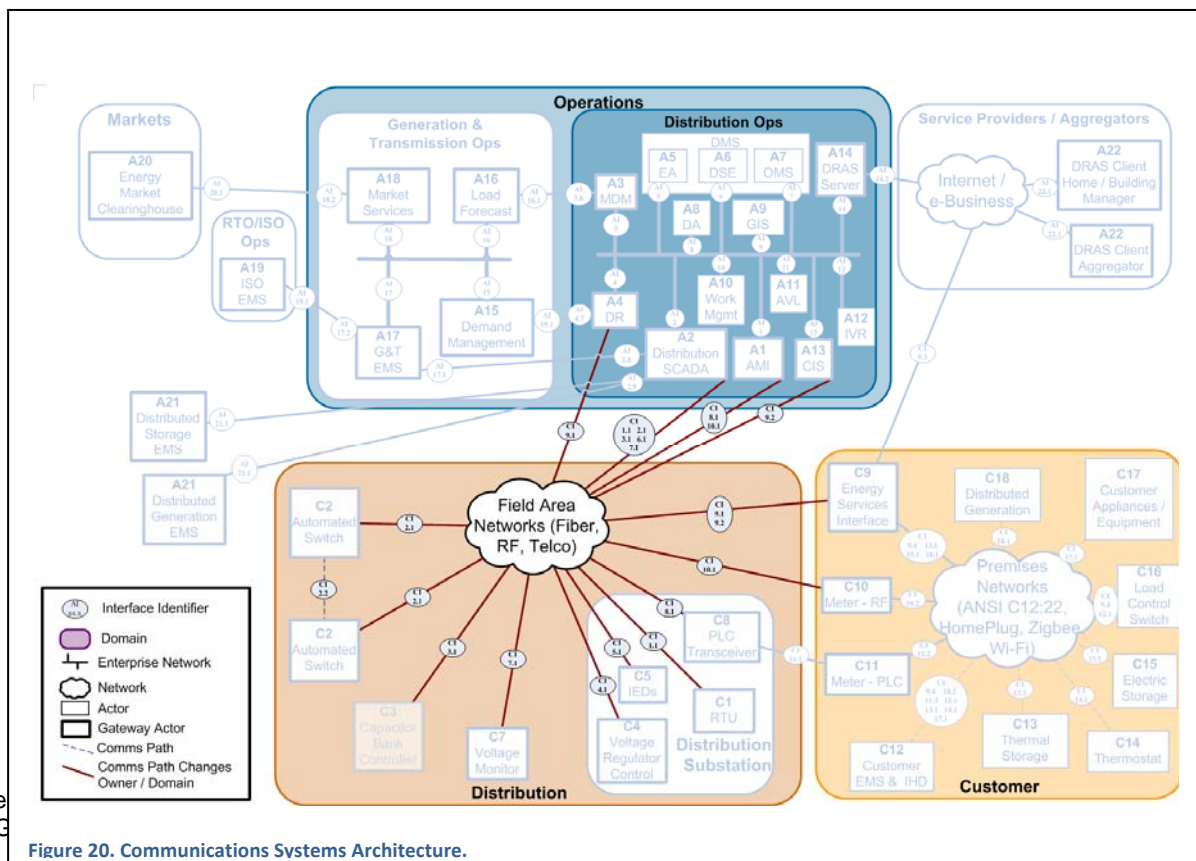
Figure 20. Communications Systems Architecture.
