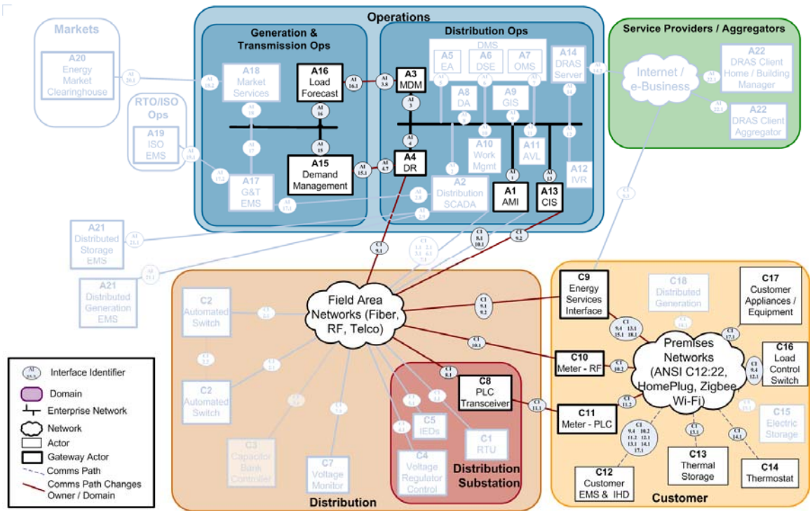
Figure 6. Smart Grid Demonstration Grant Activity Type—Demand Response over AMI.
