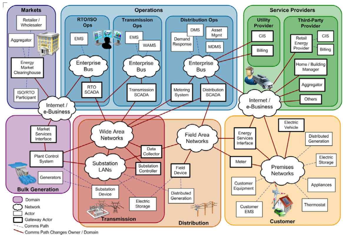
Figure 2. NIST Smart Grid Conceptual Model—Detailed View.
