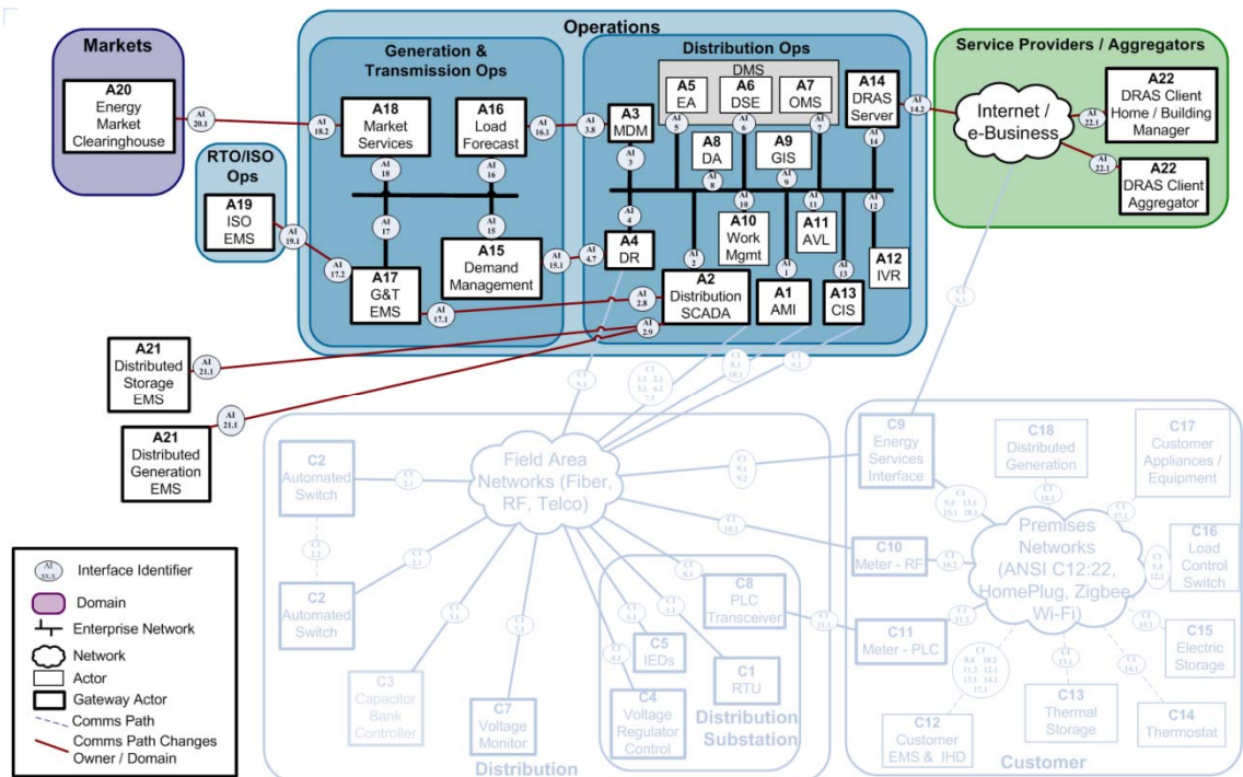
Figure 9. Project Integration Development Requirements—Enterprise Applications.
