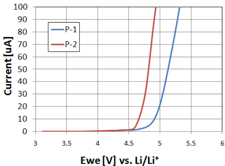
Figure 13: Cyclic voltammety results of two of Seo's catholyte polymers.
