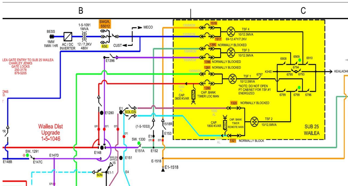
Figure 6-8: BESS circuit diagram showing connection to distribution transformer
